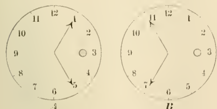
FIG. 13. ROUGH VALVE SETTING.
